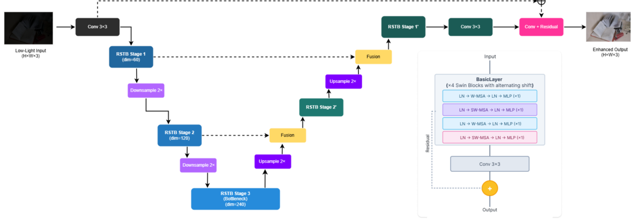
Fig. 1. Overall architecture of SwinLLIE. The network follows a U-shaped encoder-decoder structure with RSTB (Residual Swin Transformer Block) stages at three scales (dim=60, 120, 240). Skip connections with feature fusion modules preserve fine details. The right panel shows the internal structure of an RSTB block: a BasicLayer containing four alternating W-MSA (Window Multi-head Self-Attention) and SW-MSA (Shifted Window MSA) blocks, followed by a 3x3 convolution with residual connection.
