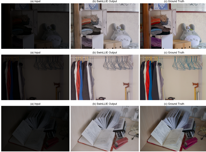
Fig. 2. Qualitative results on LOL dataset. Each row shows (a) low-light input, (b) SwinLLIE output, (c) ground truth. The proposed method effectively recovers natural illumination and colors while preserving fine details.
